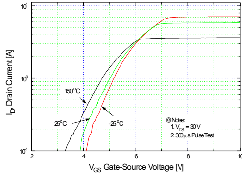
Figure 2. Transfer Characteristics
