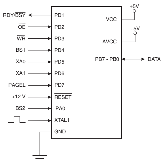
Figure 27-1. Parallel programming (1) .
