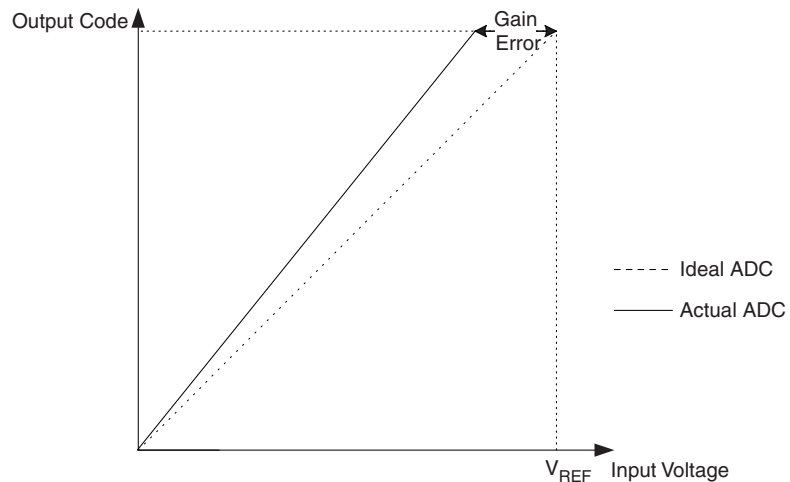
Figure 23-11. Gain error.
