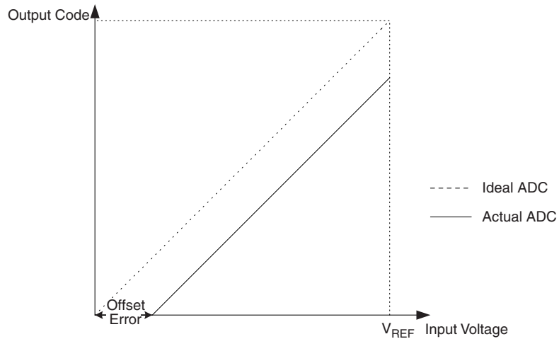
Figure 23-10. Offset error.
