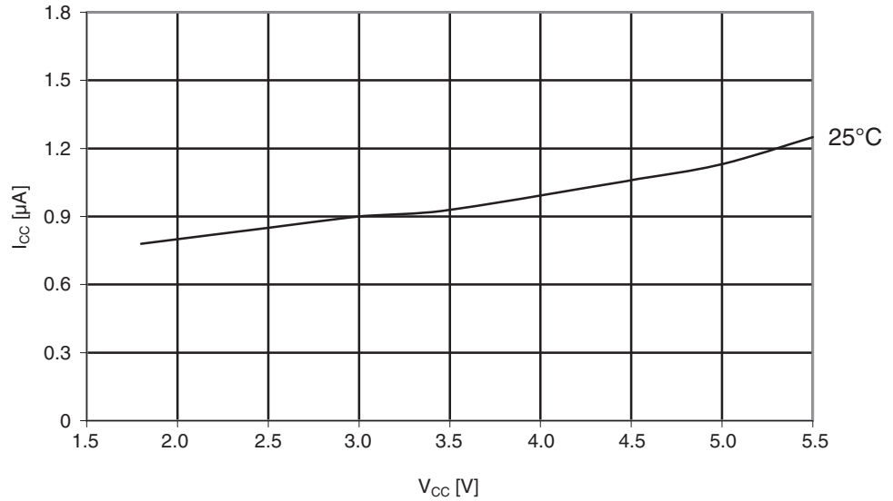
Figure 29-13. Atmel ATmega164A: Power-save supply current vs. V_{CC} (watchdog timer disabled and 32kHz crystal oscillator running).
