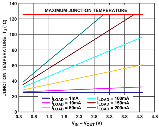
Figure 53. LFCSP 50 mm 2 of PCB Copper, T A = 25°C
