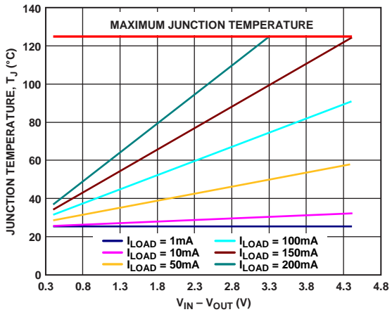
Figure 52. LFCSP 100 mm 2 of PCB Copper, T A = 25°C
