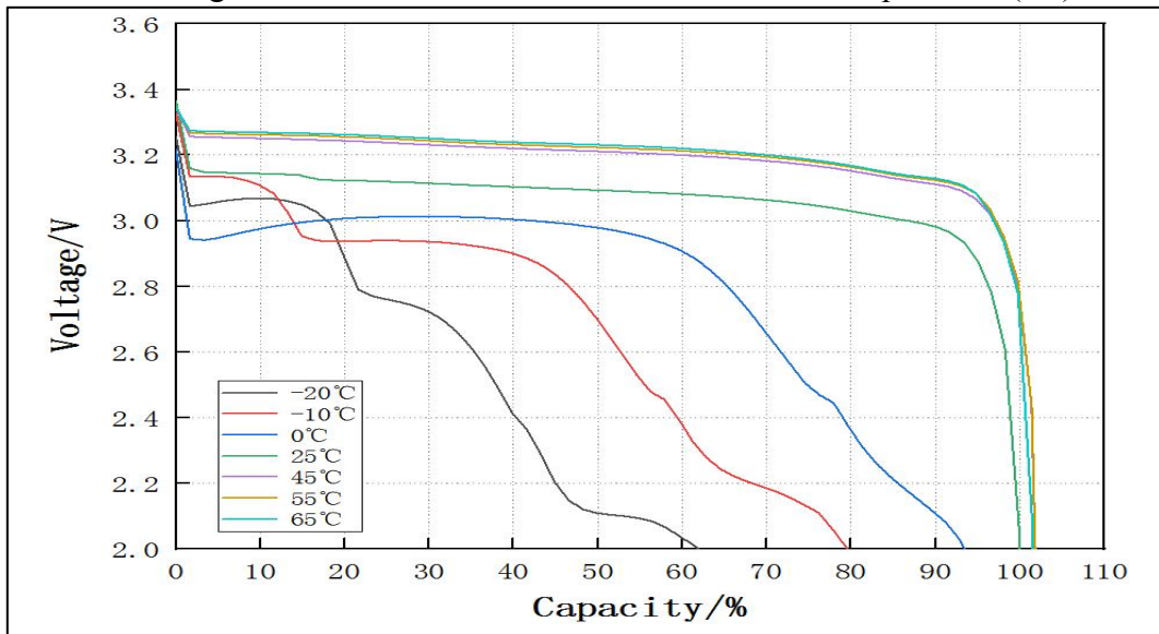
6.0 Ah 磷酸铁锂电池不同温度放电曲线 (1C) Discharge curve of 6.0 Ah LiFePO 4 cell at different temperatures(1C)
