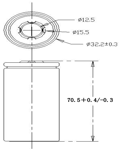
电池包膜后图片和外形尺寸 Cell's appearance and dimension with PVC sleeve
