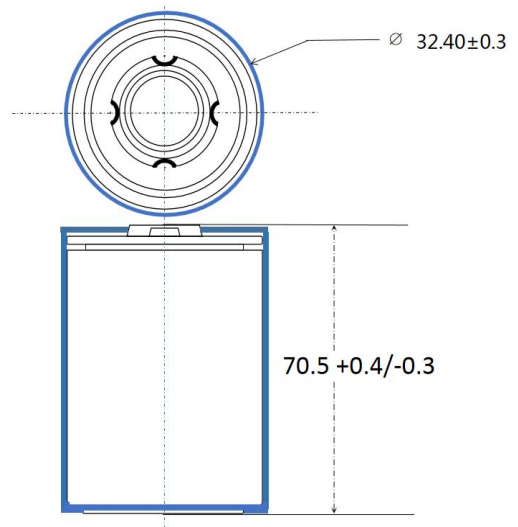
电池包膜后图片和外形尺寸 Cell's appearance and dimension with PVC sleeve
