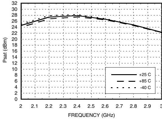
Psat vs. Temperature, Vs= 3.6V
