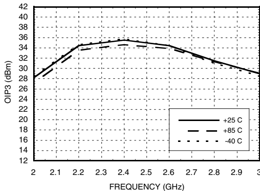
Output IP3 vs. Temperature, Vs= 3.6V
