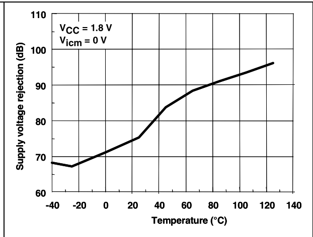
Figure 8. Supply voltage rejection vs. temperature at V_{CC} = 1.8\text{ V}
